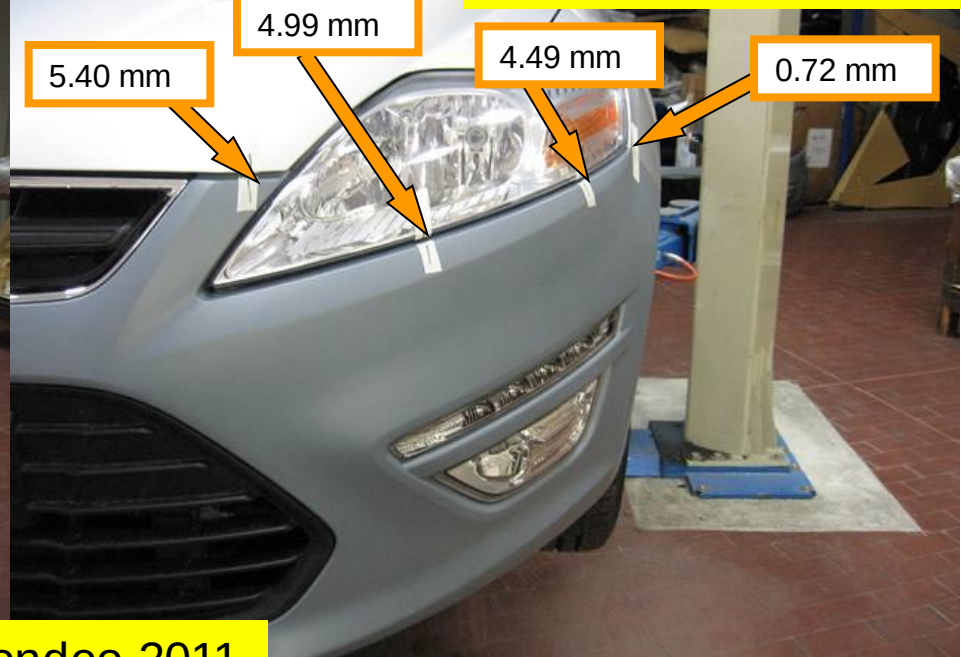
Front Bumper L/H
